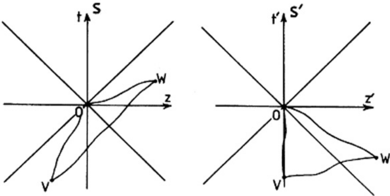
Fig. 3. Worldlines in closed Loop.
